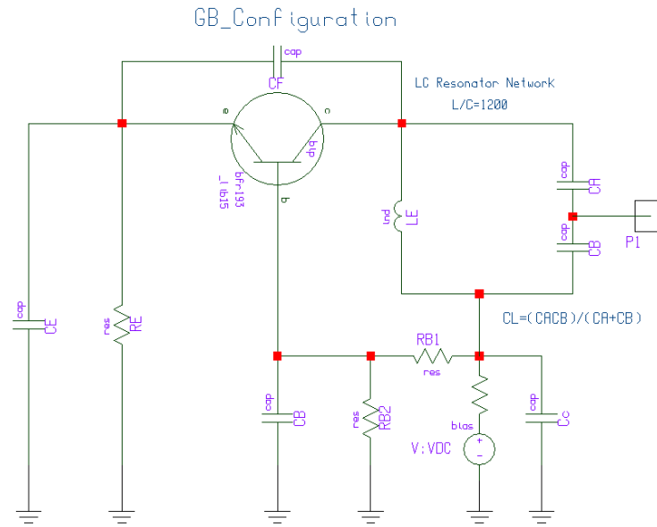
Figure 14 Typical configuration of grounded base oscillator circuit
